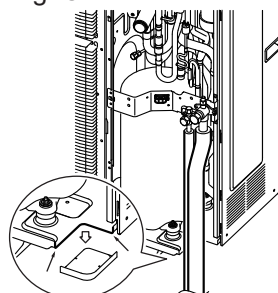
Bottom connection
