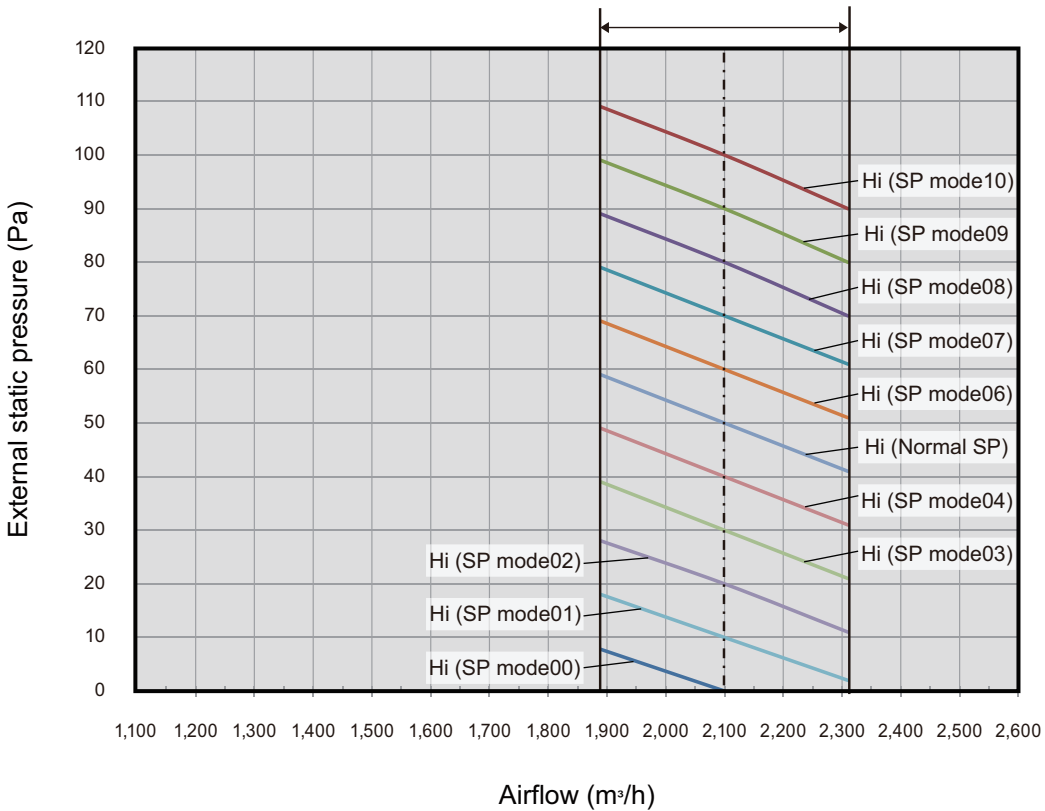
Available airflow rate @ Hi speed
