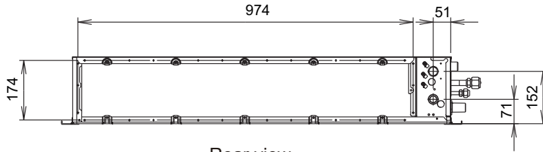
Rear view
