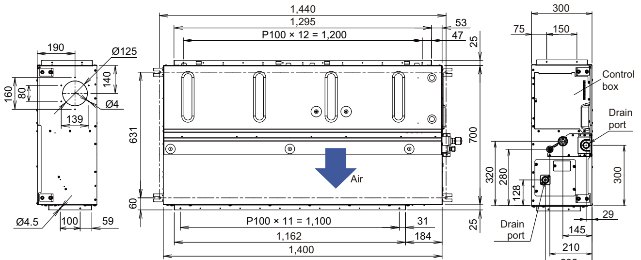
Side view (L)
