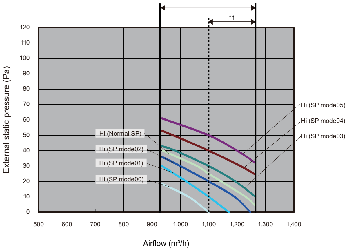
Available airflow rate range (High level)
