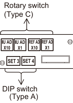
Main PCB
