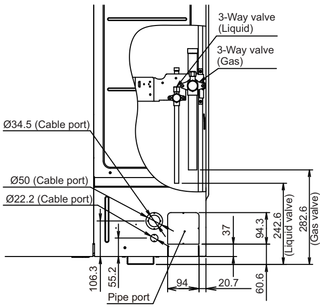
Detail A
