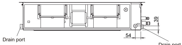
Rear view
