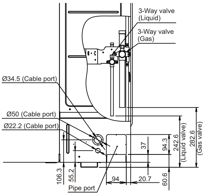
Detail A
